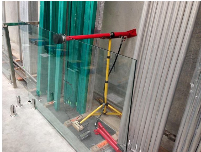
Square Core Drilled spigots under the test.
